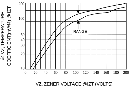
Fig. 6-UNITS 10 TO 200 VOLTS
