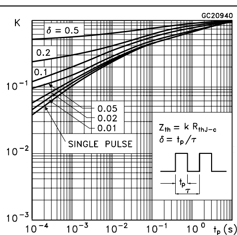
Figure 6. Thermal impedance for DPAK / IPAK
