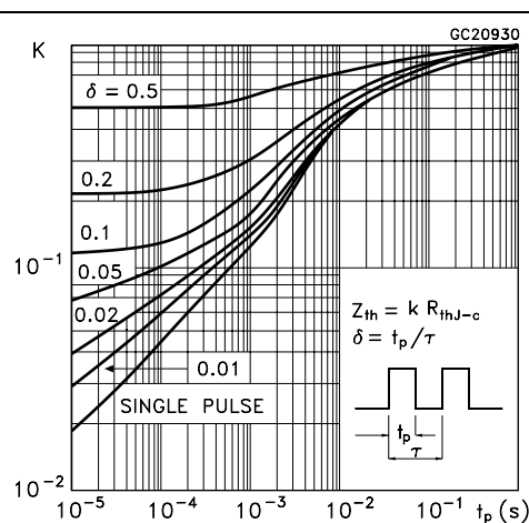
Figure 4. Thermal impedance for TO-220FP
