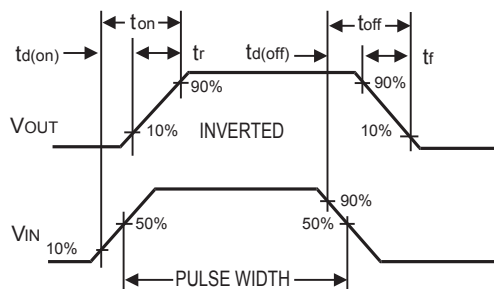
Figure 10. Switching Waveforms
