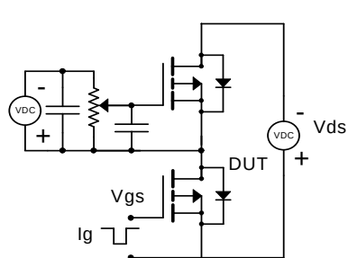
Gate Charge Test Circuit &amp; Waveform
